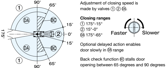
Range of delayed action and back check
