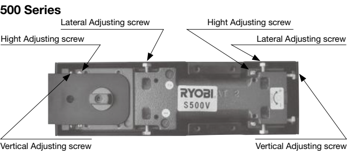
Adjustable range for closing position and clearance
