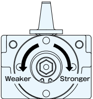
How to adjust closing power
