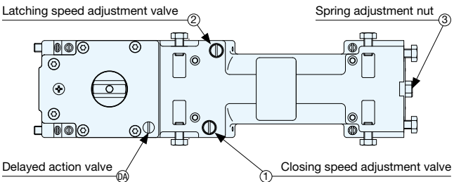
Position of valves
