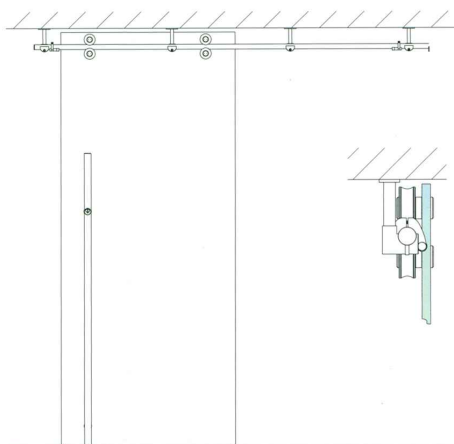
2. mounting to roof
