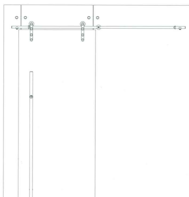
2. front mounting to glass wall
