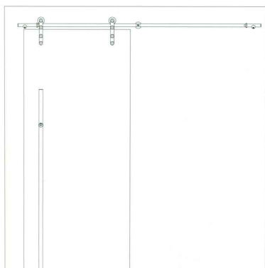
1. front mounting to brick wall or wood wall
