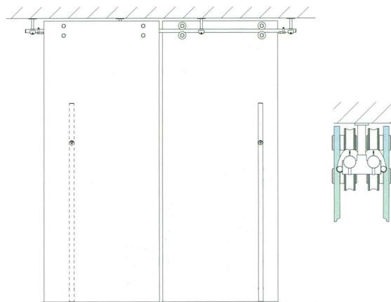
3. mounting to roof, double door
