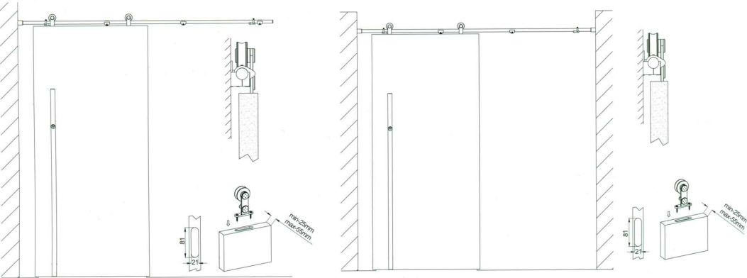
3.front mounting and side mounting to brick wall or wood wall
